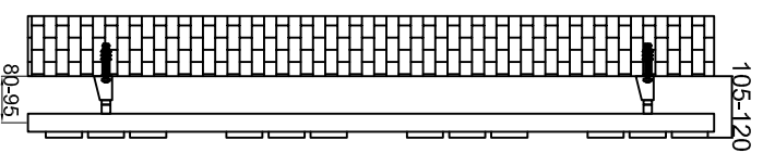
Side View
